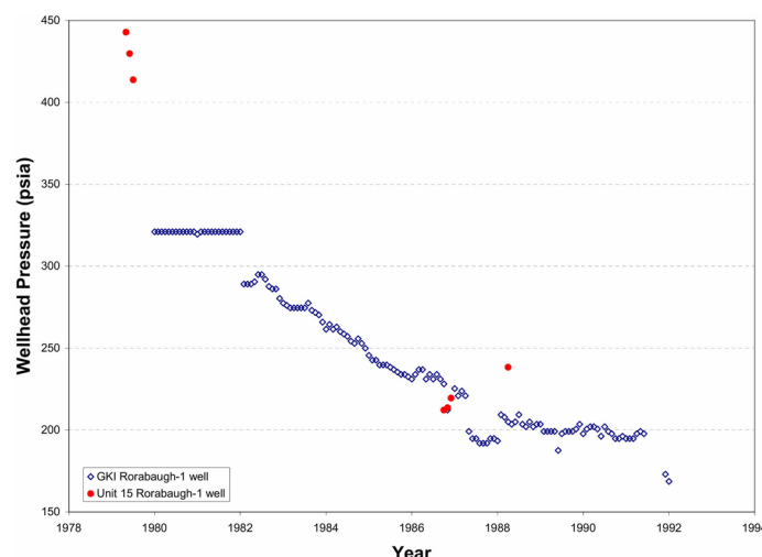
Figure 6. Static Wellhead Pressure History in the Unit 15 Area (From Sanyal, et al., 2008).
