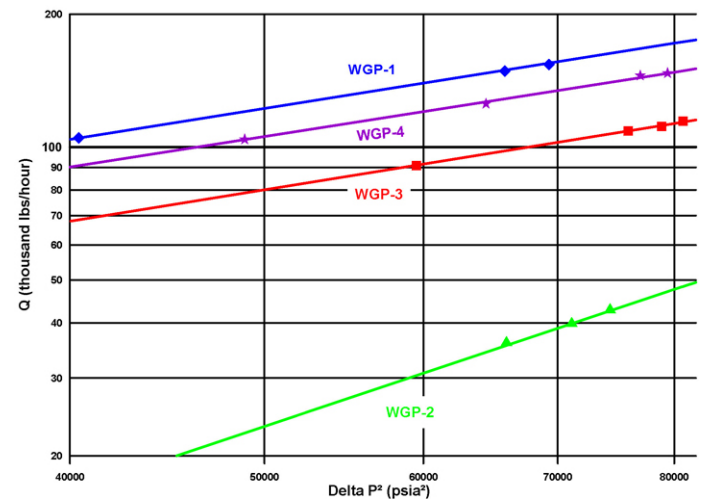
Figure 9. Well Deliverability Plots.
