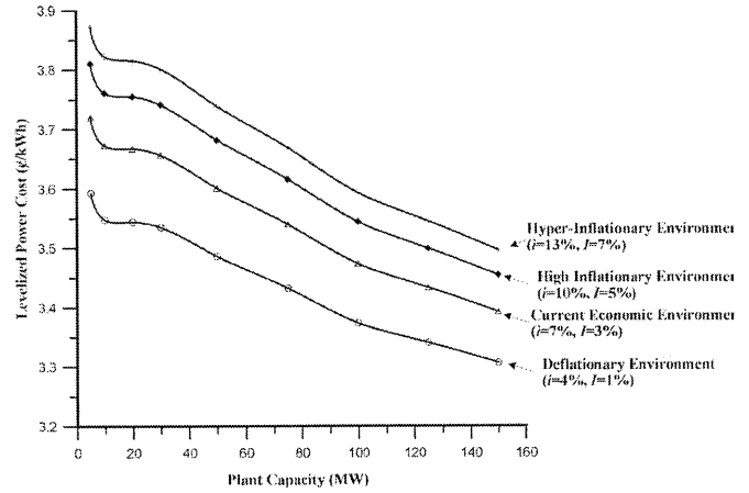
Figure 6. Levelized power cost versus plant capacity under various macro-economic conditions (for 20 years of make-up well drilling).
