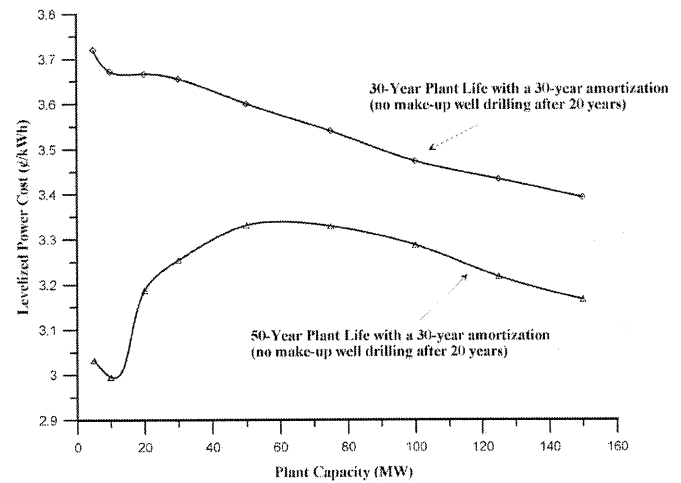
Figure 7. Effect of plant life on levelized power cost (20 years of make-up well drilling).
