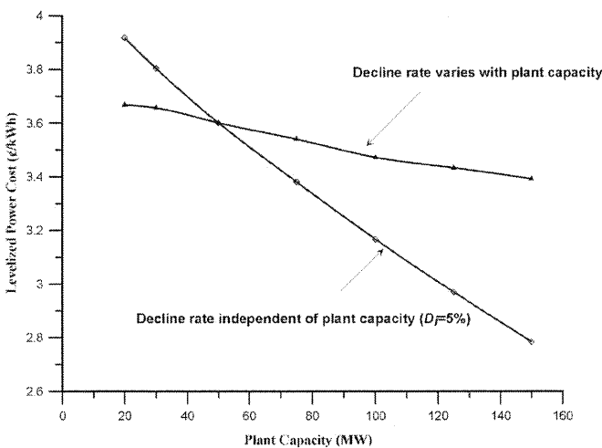
Figure 8. Levelized power cost versus plant capacity (for 20 years of make-up well drilling).
