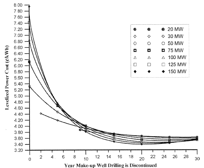
Figure 2. Levelized power cost versus the year make-up well drilling is discontinued.
