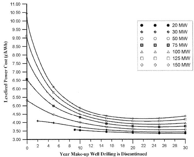
Figure 9. Levelized power cost versus the year make-up well drilling is discontinued ("no economy of scale" case).
