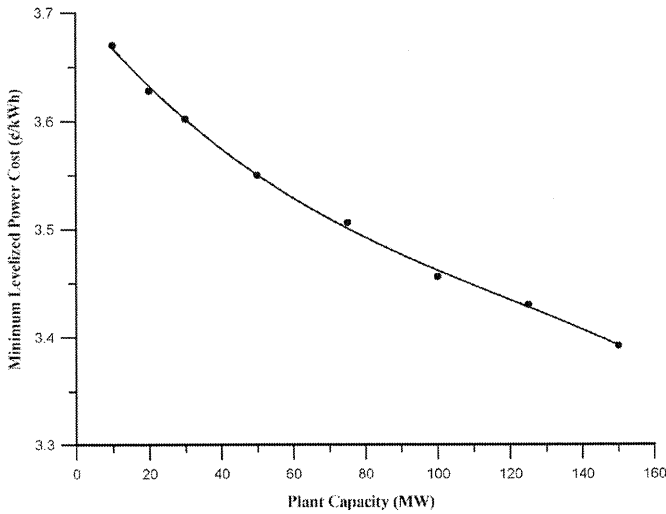
Figure 3. Minimum levelized power cost versus plant capacity.
