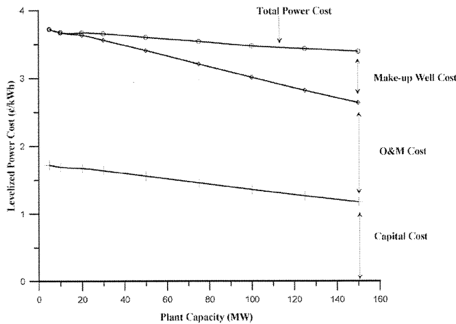
Figure 4. Components of levelized power cost versus plant capacity (assuming 20 years of make-up well drilling).
