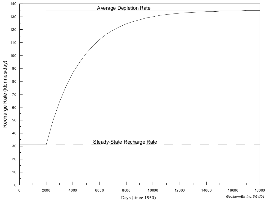
Figure 7. Recharge versus time, Wairakei field
