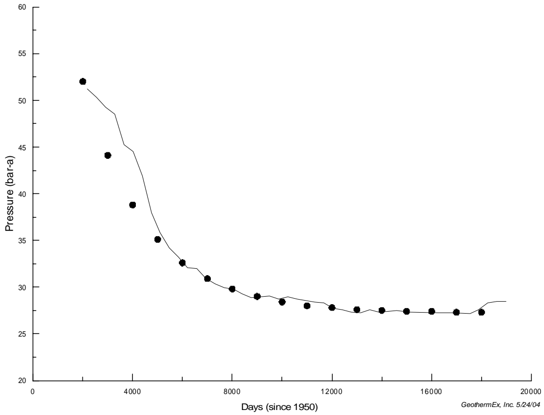
Figure 6: Observation and computed liquid pressures, Western Borefield
