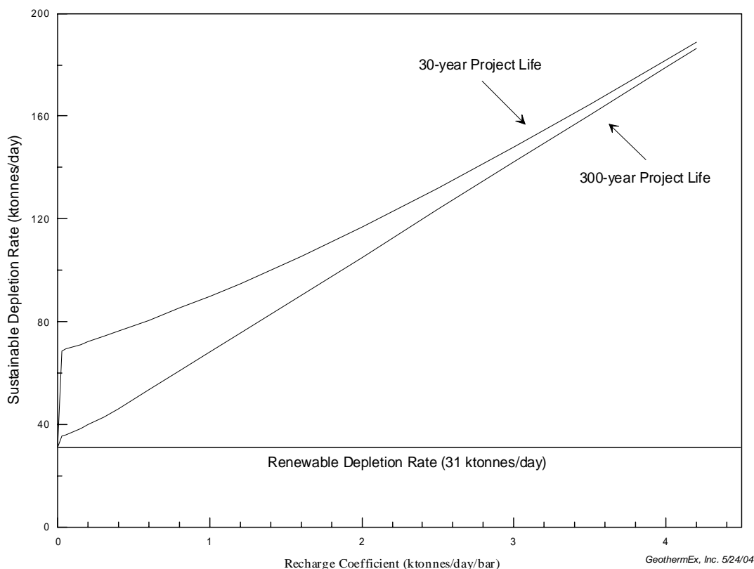
Figure 9: Sustainable capacity versus recharge coefficient
