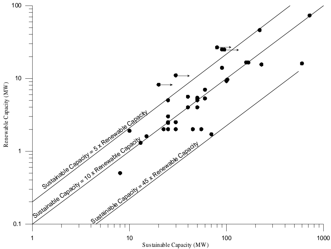
Figure 3: Renewable capacity versus sustainable capacity
