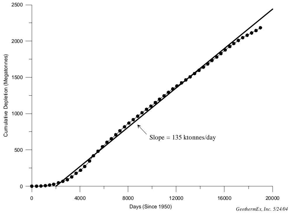
Figure 5: Cumulative depletion history
